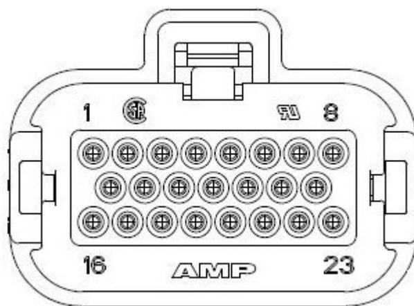
Conector Ampseal
