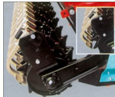
Rullo paker/ Raschiatore regolabile. Paker roller/ Adjustable scraper. Rouleau paker/ Racleur réglable. Paker-Walze/einstellbarer Schaber.
